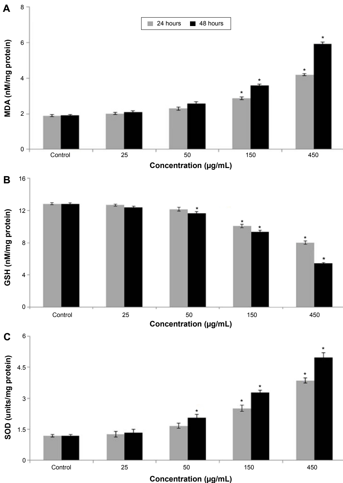
Figure 5 Al 2 O 3 NP-induced oxidative stress.
