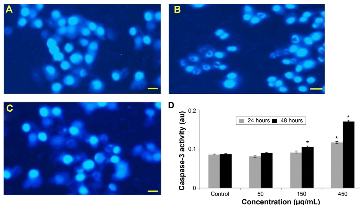
Figure 6 Chromosomal condensation and induction of caspase-3 activity in HepG2 cells after treatment with \text{Al}_2\text{O}_3 NPs.
