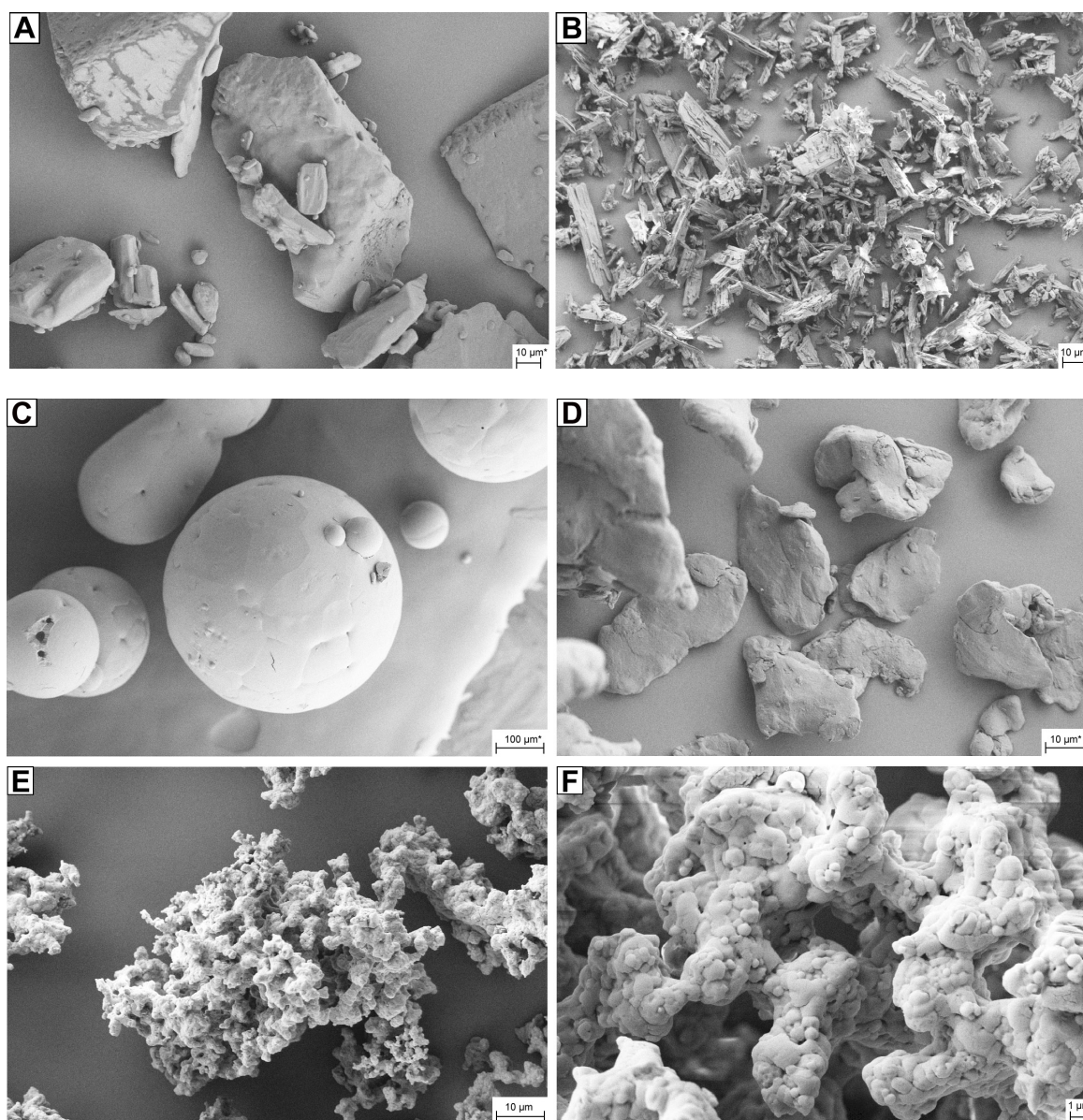
Figure 3 The surface morphology of LAA (A), ITZ (B), F127 (C), HPMC (D), SD particles (E and F) observed by SEM.
