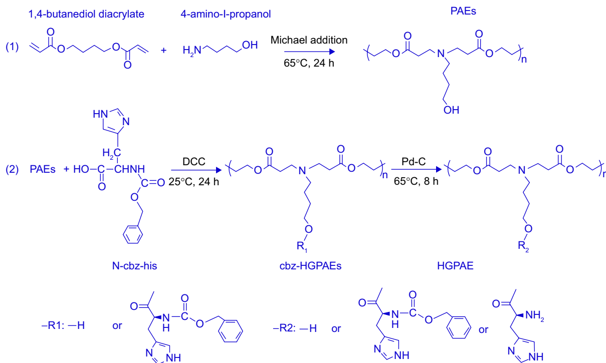
Figure 2 The synthesis process of PAEs and HGPAE.
