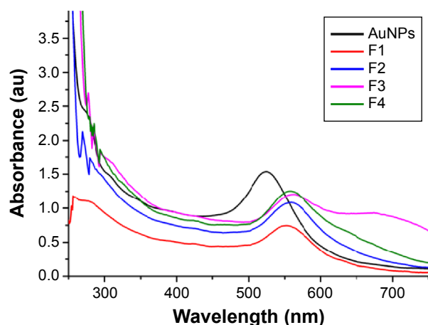
Figure 1 Visible absorption spectra for AuNPs without glucosamine and AuNPs functionalized with different concentrations of glucosamine, ie, (F1) 0.021% w/v, (F2) 0.043% w/v, (F3) 0.086% w/v, and (F4) 0.12% w/v.
