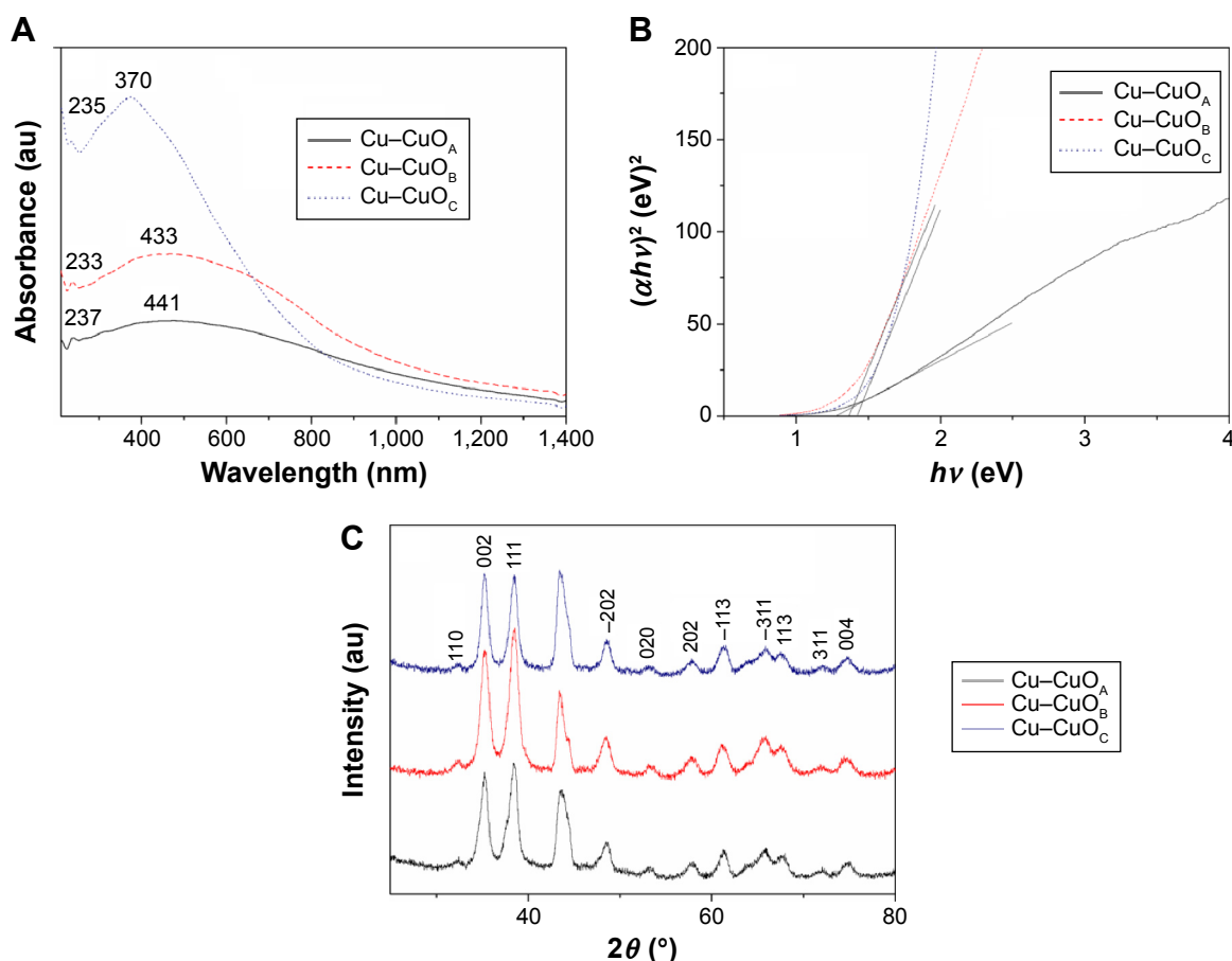
Figure 4 Optical and structural characteristics of Cu–CuO.
