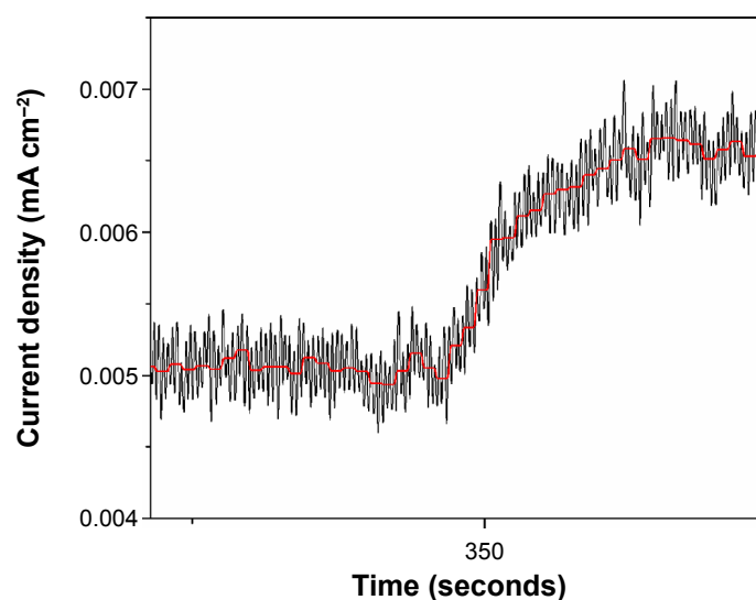
Figure S3 A typical amperometric response curve obtained for 2 \mu\text{M} glucose of the ITO/MWCNT/Cu-CuO 8 electrode.
