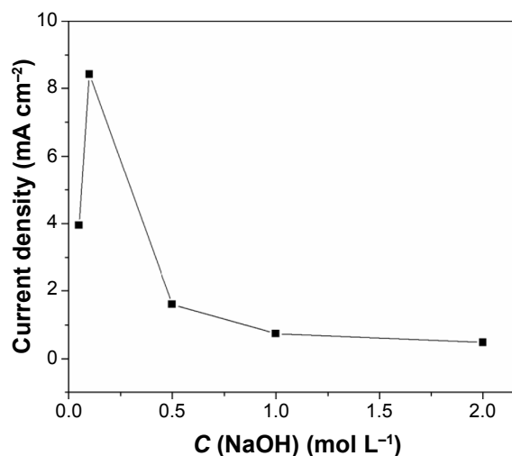
Figure 8 Effect of NaOH concentration on the current density (at +0.9 V) measured for ITO/MWCNT/Cu-CuO 8 electrode in a 10 mM glucose solution.
