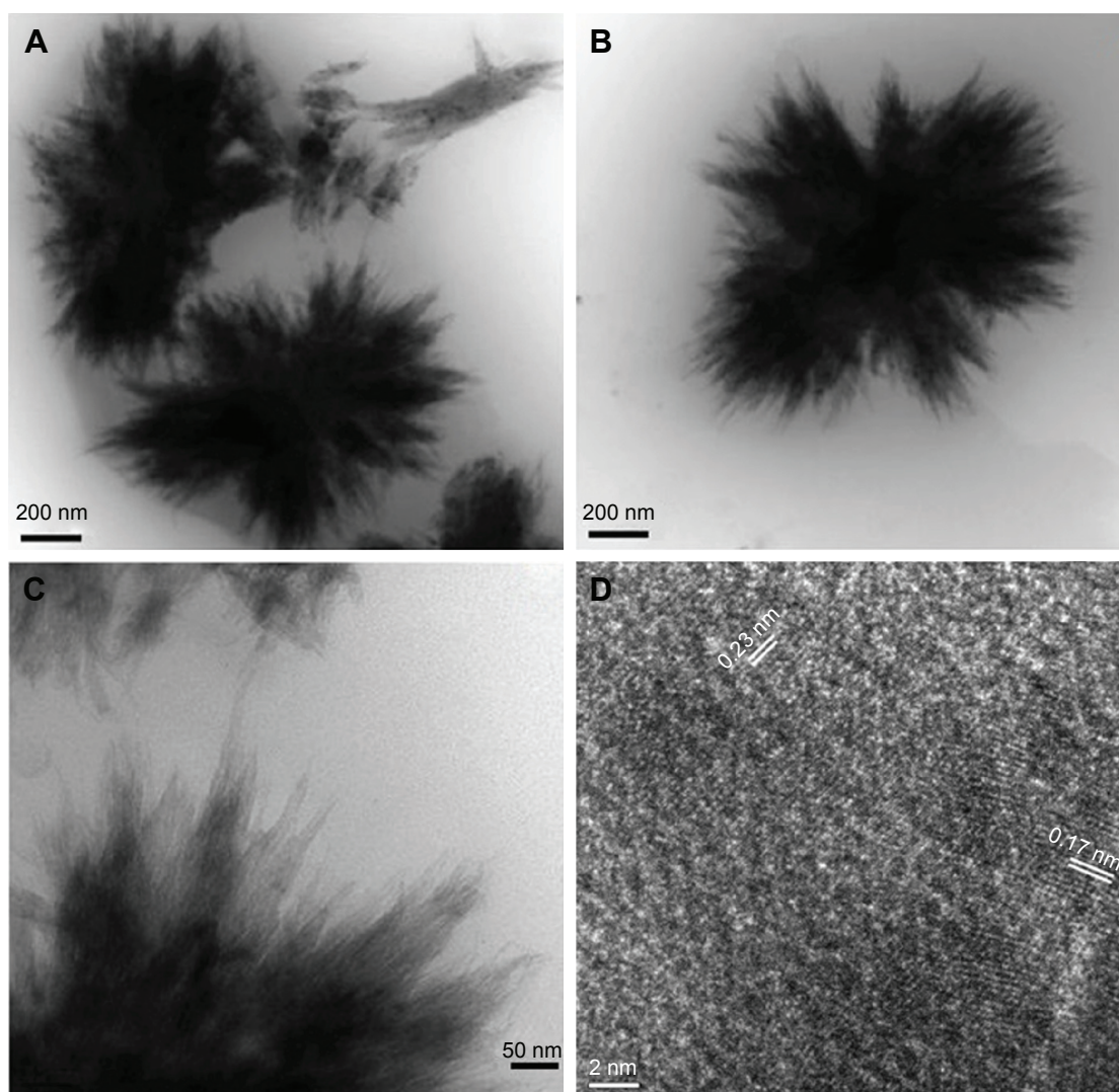
Figure 3 Transmission electron microscopy micrographs. Notes: (A–C) Cu–CuO x . (D) Lattice fringe pattern of Cu–CuO.
