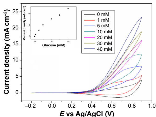
Figure 7 Cyclic voltammogram obtained at 20 \text{ mV s}^{-1} for ITO/CNT/Cu-CuO 8 at different glucose concentrations in 0.1 M NaOH.
