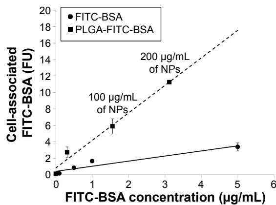
Figure 3 Flow cytometry analysis of cellular uptake.
