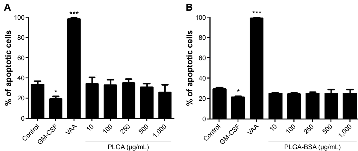
Figure 6 Effects of NPs on neutrophil apoptosis.
