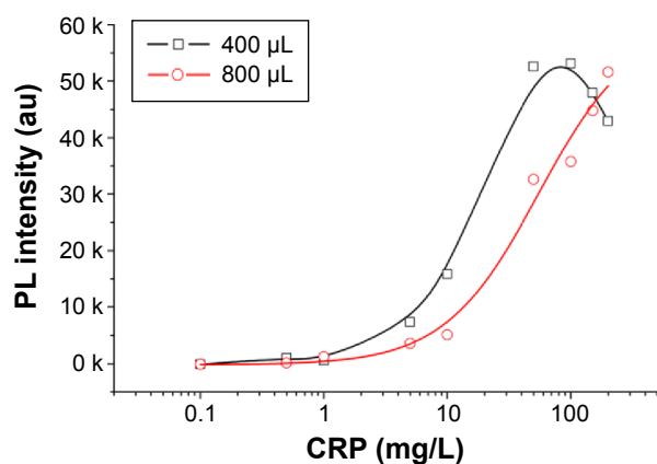
Figure 6 The quantitative dynamic range of the developed QDs-based immunofiltration assay using different volume of QDs conjugates.
