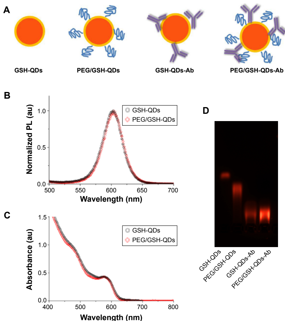
Figure 2 Synthesis and characterization of PEGylated QDs and QD-antibody conjugates.
