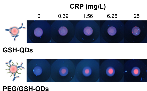
Figure 3 Comparative detection of CRP using QDs labeling conjugates prepared from GSH-QDs and PEG/GSH-QDs conjugates.
