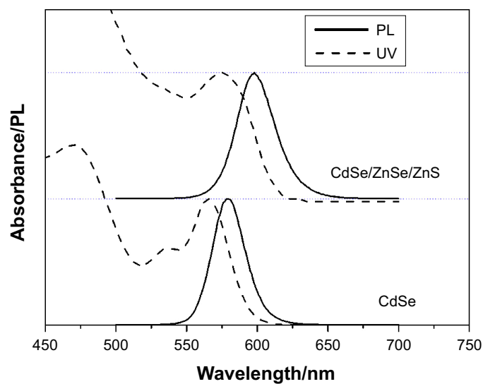
Figure S1 UV-Vis absorbance and fluorescent spectra of CdSe core and CdSe/ZnSe/ZnS core/shell/shell QDs.
