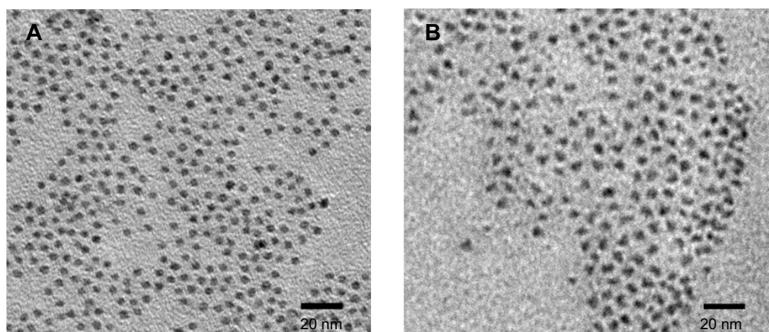
Figure S2 TEM graphs of CdSe core (A) and CdSe/ZnSe/ZnS core/shell/shell (B) QDs.
