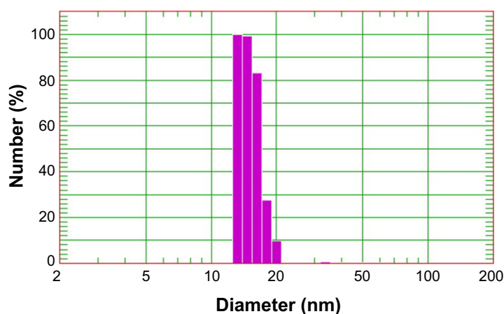
Figure S4 Dynamic light scattering analysis of PEG/GSH-QDs.
