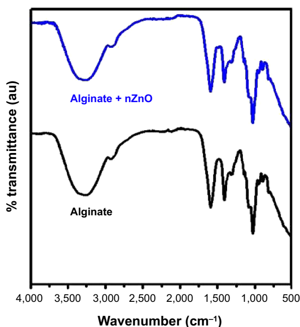
Figure 3 FTIR image of alginate control and alginate + nZnO bandages.
