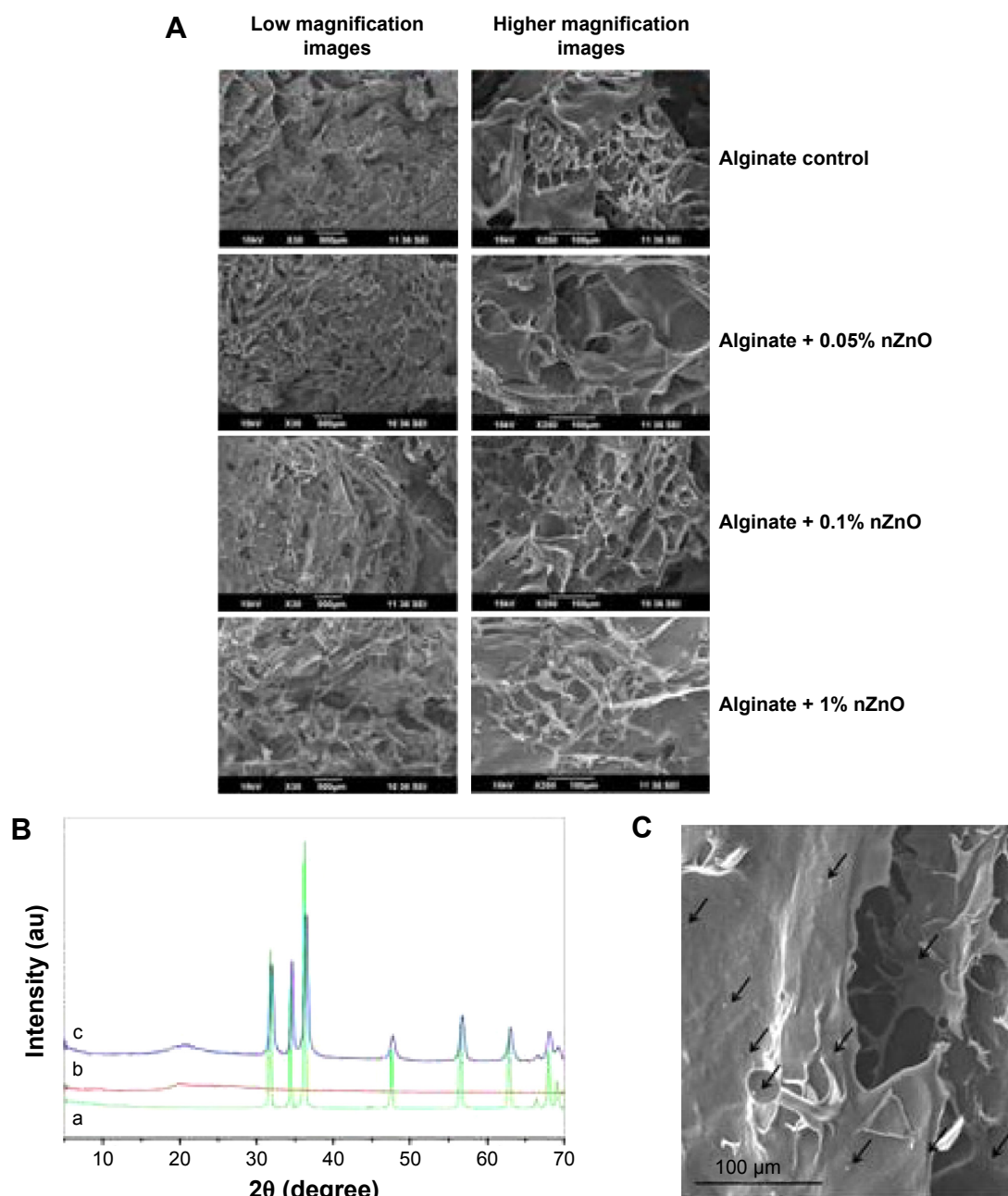
Figure 2 Physico-chemical characterization of alginate hydrogel/nZnO composite bandages.
