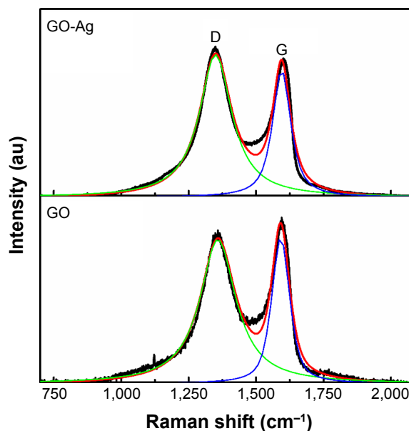
Figure S4 Raman spectra of GO and GO-Ag nanocomposites.
