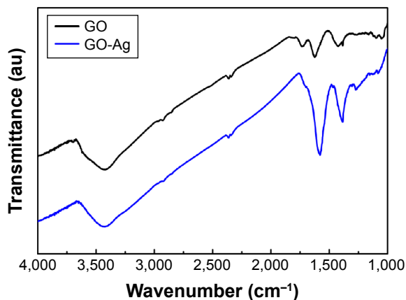
Figure S3 FTIR spectra of GO and GO-Ag nanocomposites.
