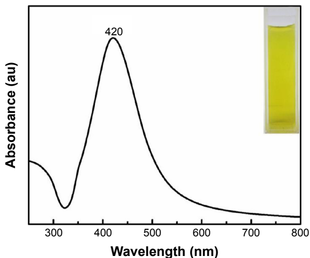
Figure S5 UV-vis absorption spectrum of bare AgNPs.
