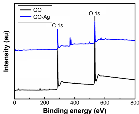
Figure S2 XPS survey spectra of GO and GO-Ag nanocomposite.
