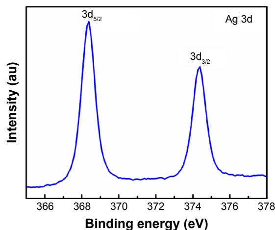
Figure S1 Ag 3d XPS spectrum of GO-Ag nanocomposite.
