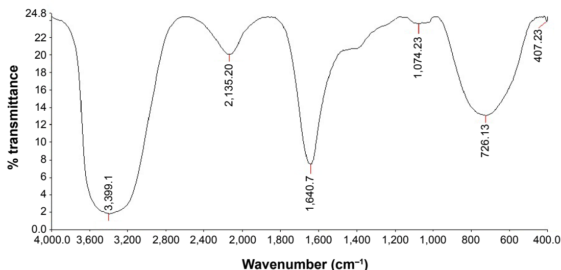
Figure 3 FTIR spectrum for Rosa damascena extract.
