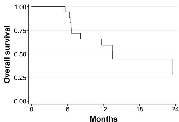
Figure 1 Median overall survival in the entire population.
