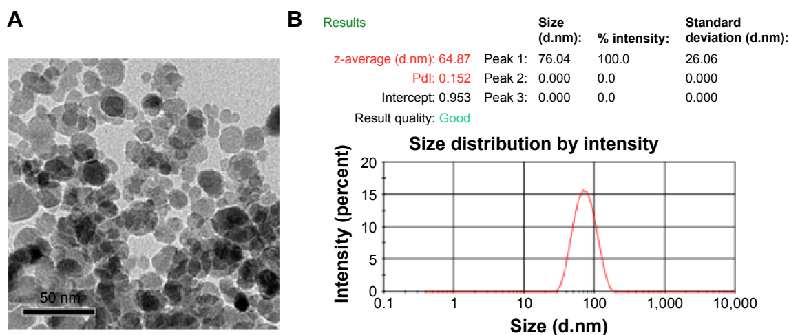
Figure 1 Characterization of \text{Fe}_3\text{O}_4 .
