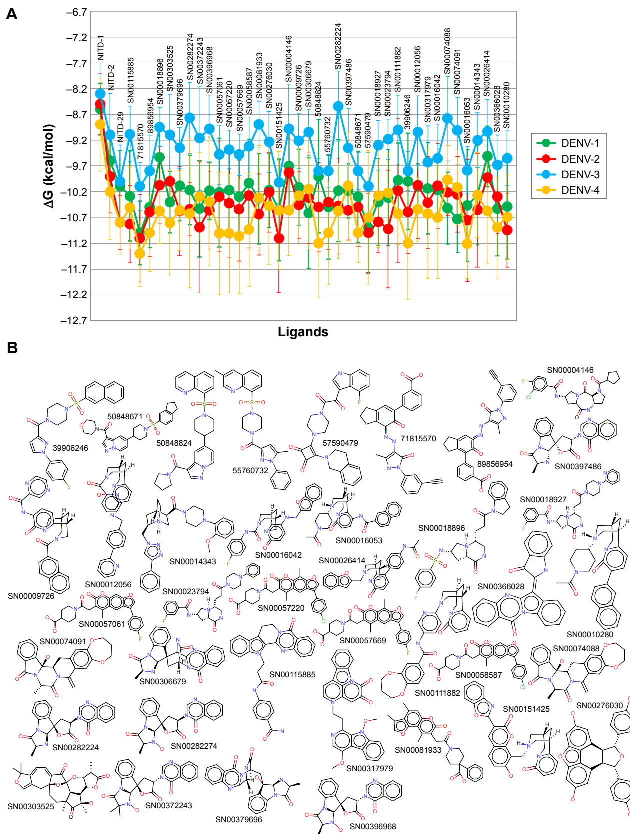
Figure 2 Comparison of the free energy variation ( \Delta G ) for selected compounds based on molecular docking analysis against NS5 RdRps of all four serotypes of dengue virus (A). \Delta G for NITD compounds is also included. (B) The molecular structures of the compounds represented in (A); the PubChem ID or the SuperNatural 2 ID is close to the structure of each compound.
