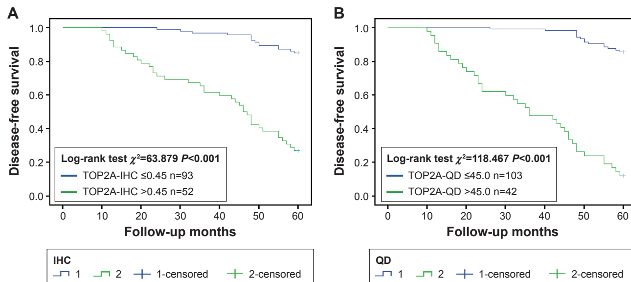
Figure 6 Cumulative 5-DFS curves according to TOP2A-IHC (A) and TOP2A-QD (B), respectively.
