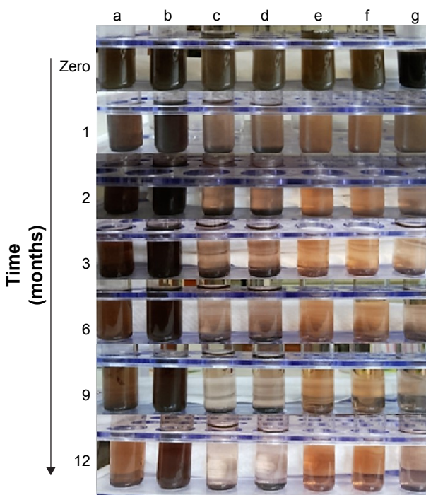
Figure 4 Effect of coating type on AgNPs ( 500\text{ }\mu\text{g AgNPs/mL} ) sedimentation rate in water over time: (a) 5 mM PEG-coated AgNPs; (b) 10 mM PEG-coated AgNPs; (c) 5 mM SDS-coated AgNPs; (d) 10 mM SDS-coated AgNPs; (e) 5 mM \beta -CD-coated AgNPs; (f) 10 mM \beta -CD-coated AgNPs; and (g) uncoated AgNPs.
