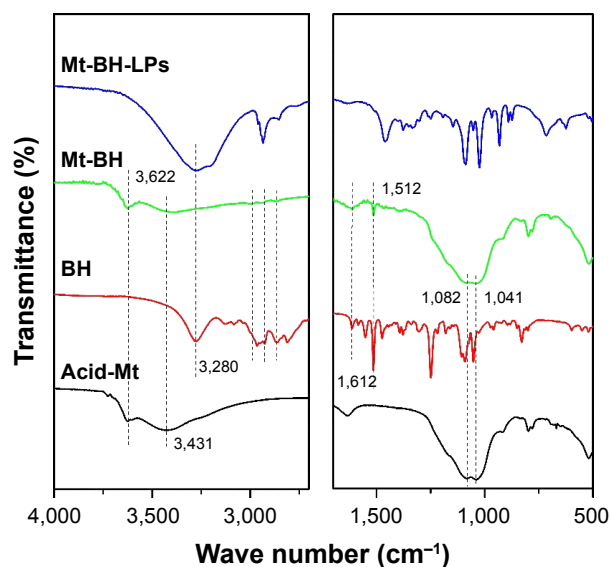
Figure 8 FTIR spectra of acid-Mt, BH, Mt-BH, and Mt-BH-LPs.
