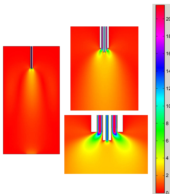
Figure 9 Velocity field of convex nozzle at CO 2 flow rate of 4.5 kg/h.
