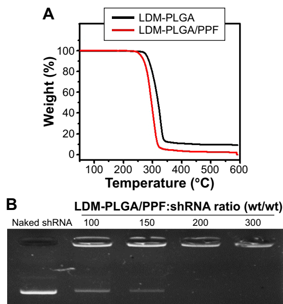
Figure 3 (A) Thermogravimetric analysis of LDM-PLGA and LDM-PLGA/PPF. (B) Agarose gel electrophoresis assay of LDM-PLGA/PPF/VEGF shRNA at various weight ratios of LDM-PLGA/PPF to VEGF shRNA.
