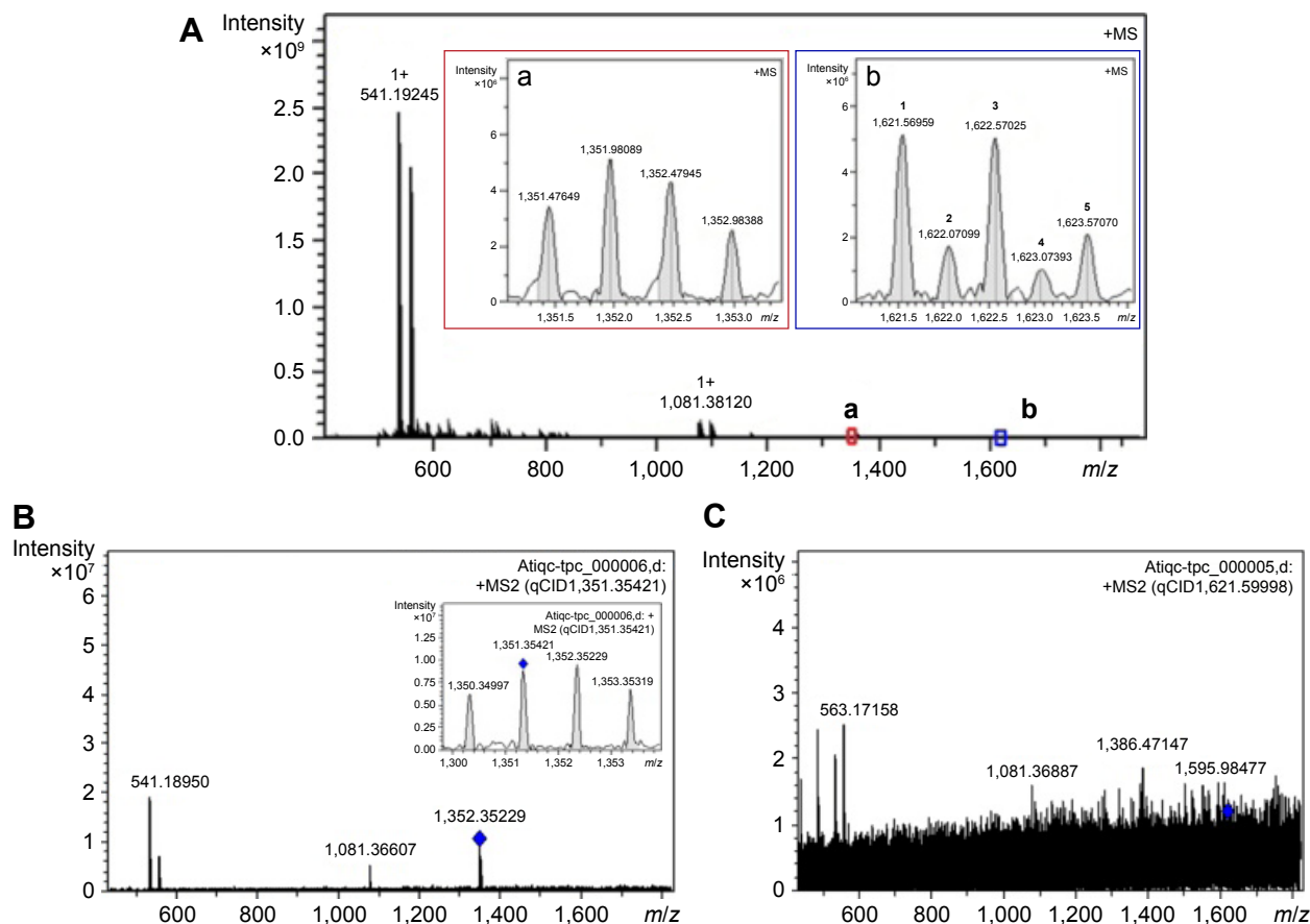
Figure 2 FT-MS and qCID spectra of ATIQCTPC.
