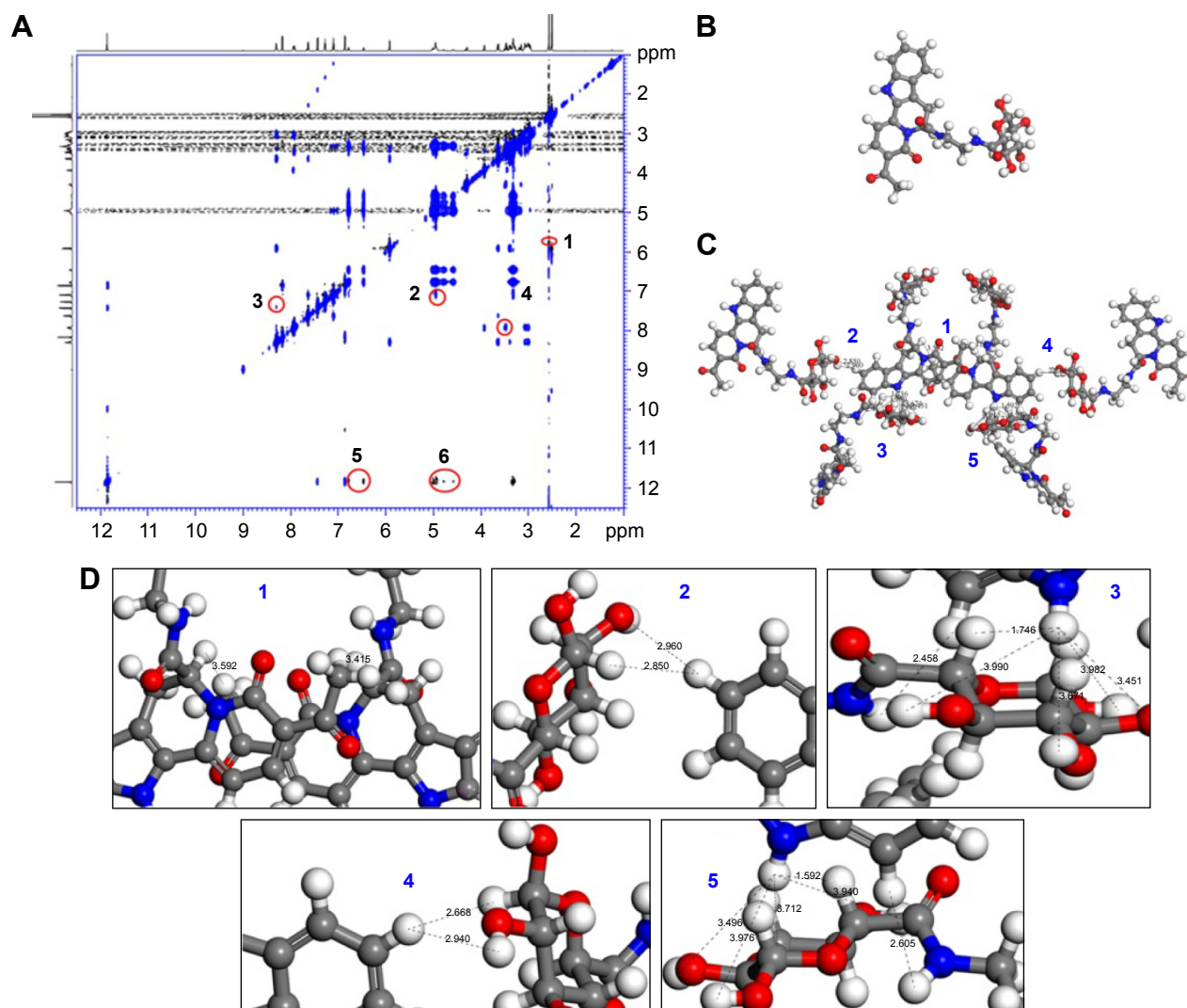
Figure 3 ROESY 2D ^1\text{H} NMR spectrum, the monomer, and the hexamer conformations of ATIQCTPC.
