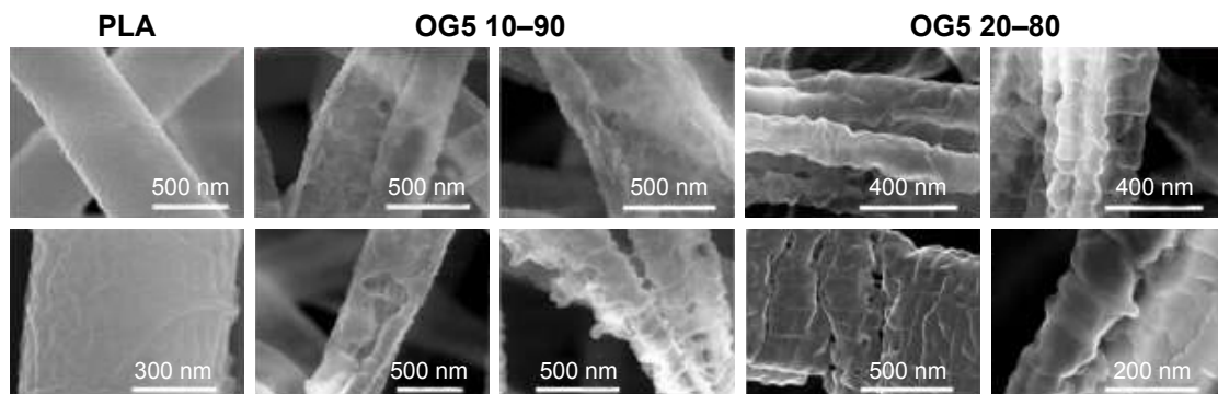
Figure 2 Images of typical defects observed on the PLA and hybrid fibers after 28 days of incubation in SBF.
