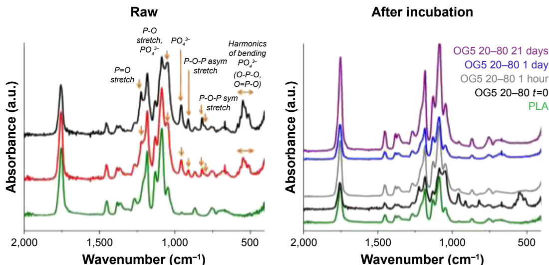
Figure 5 FTIR spectra of the PLA and hybrid fibers as produced by electrospinning (Raw) and during the degradation test (PLA spectra is added for comparison). Abbreviations: FTIR, Fourier-transform infrared spectroscopy; PLA, polylactic acid.
