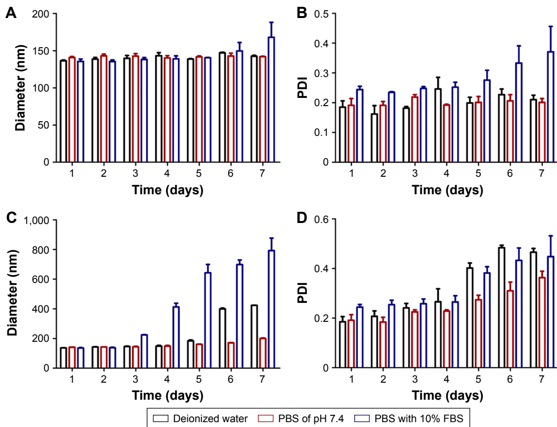
Figure 2 Colloidal stability of FA-PPLNPs/Mtx in different media.
