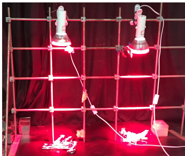
Figure S2 Photo of external NIR emitter with a power density of 10 \text{ mW/cm}^2 .
