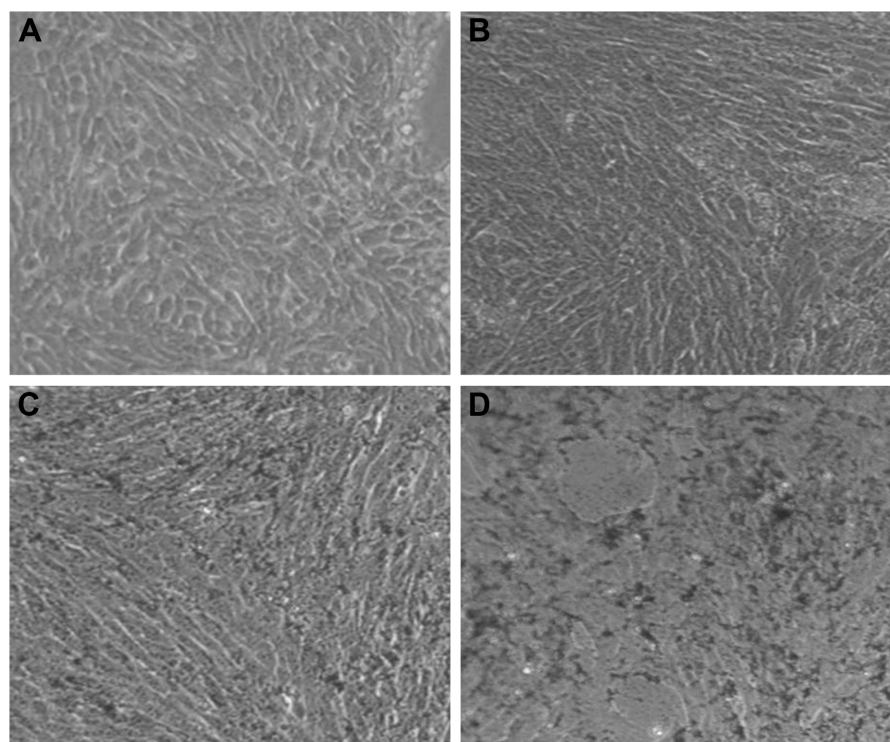
Figure 10 Microscopic images of 4T1 cells: (A) untreated and treated with (B) 5 \mu\text{g/mL} , (C) 20 \mu\text{g/mL} and (D) 50 \mu\text{g/mL} BSeNPs.
