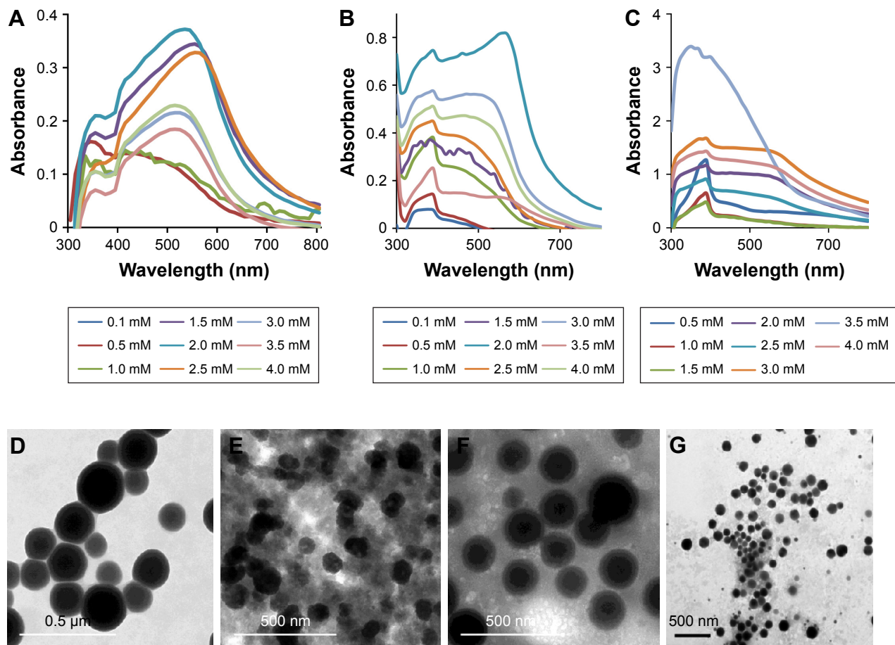
Figure 4 UV-Vis spectrum of SeNPs synthesized by total cell protein using (A) 1 mg/mL, (B) 2 mg/mL and (C) 3 mg/mL. TEM micrographs of SeNPs synthesized by TCP using (D) 1 mg/mL at 2 mM \text{Na}_2\text{SeO}_3 concentration, (E) 1 mg/mL at 4 mM \text{Na}_2\text{SeO}_3 concentration, (F) 2 mg/mL at 2 mM \text{Na}_2\text{SeO}_3 concentration and (G) 3 mg/mL at 3.5 mM \text{Na}_2\text{SeO}_3 concentration.
