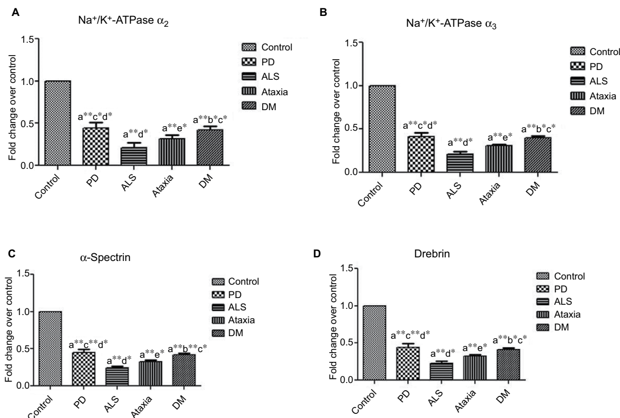
Figure 3 Data on qRT PCR analysis between control and neurodegenerative subjects: (A) NKA \alpha_2 , (B) NKA \alpha_3 , (C) SPTA and (D) drebrin. ANOVA was performed using the mean fold change ( p \leq 0.05 ) compared with (a) control, (b) Parkinson's disease, (c) amyotrophic lateral sclerosis, (d) ataxia and (e) dementia. Error bars indicate SEM. * p \leq 0.05 indicates significance; ** p \leq 0.01 indicates highly significant.
