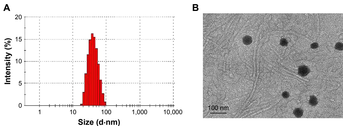
Figure 1 Size distribution of optimized CK-M (A). Transmission electron micrographs of optimized CK-M. Scale bar = 100 nm (B). Abbreviation: CK-M, ginsenoside-compound-K-loaded TPGS/PEG-PCL mixed micelles.
