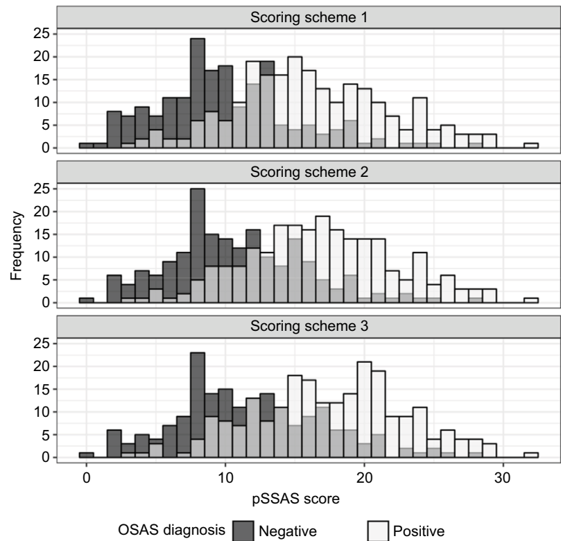
Figure 2 Frequency distribution of the pSSAS questionnaire scores for individuals according to OSAS diagnosis. Notes: White = individuals with OSAS; black = individuals without OSAS; gray = overlap of the columns. Abbreviations: pSSAS, pictorial Sleepiness and Sleep Apnoea Scale; OSAS, obstructive sleep apnea syndrome.
