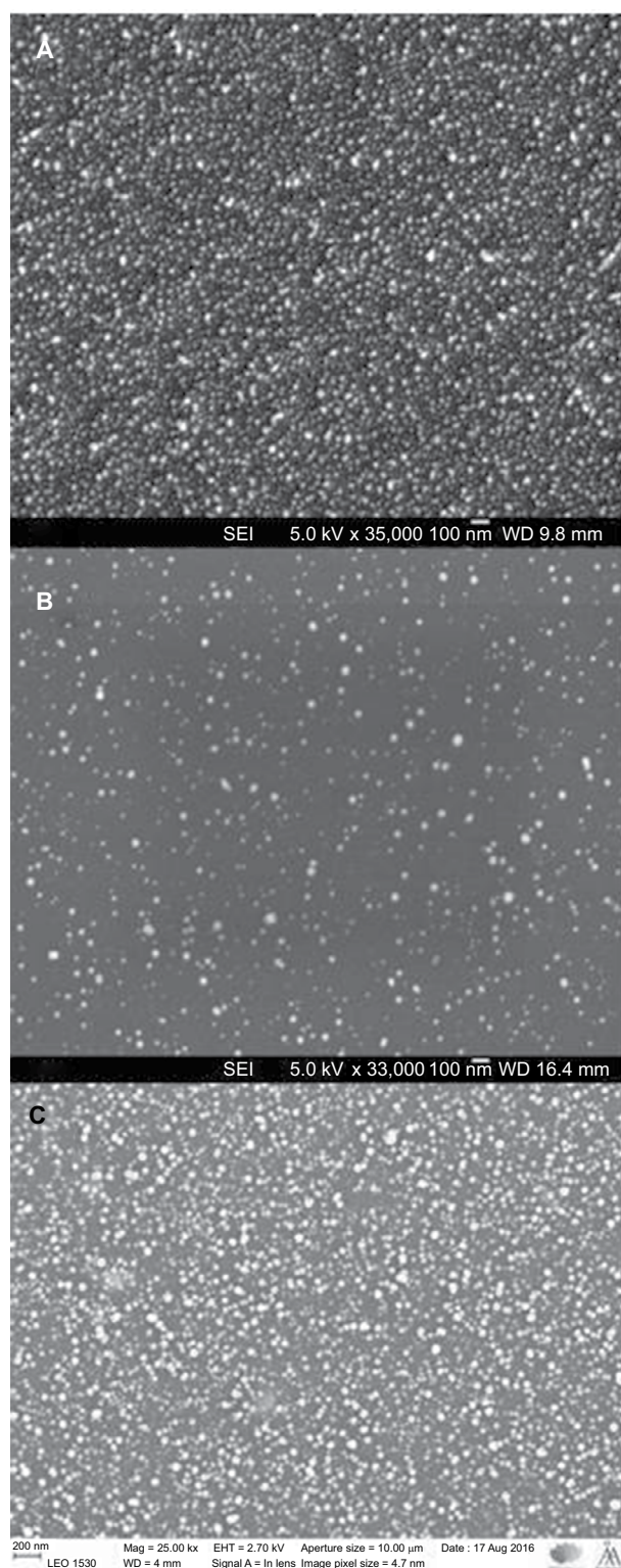
Figure 5 SEM image showing silver nanoparticles on the glass surface with direct 30× (A) and indirect 30 s (B) deposition, and direct 30× deposition on PET surface (C). Abbreviations: PET, polyethylene terephthalate; SEM, scanning electron microscopy; SEI, secondary electron imaging; WD, working distance; EHT, electron high tension.
