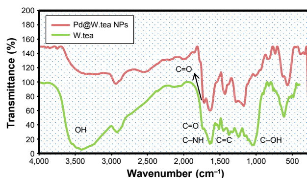
Figure 3 FTIR spectra of Pd@W.tea NPs and white tea (W.tea) extract.
