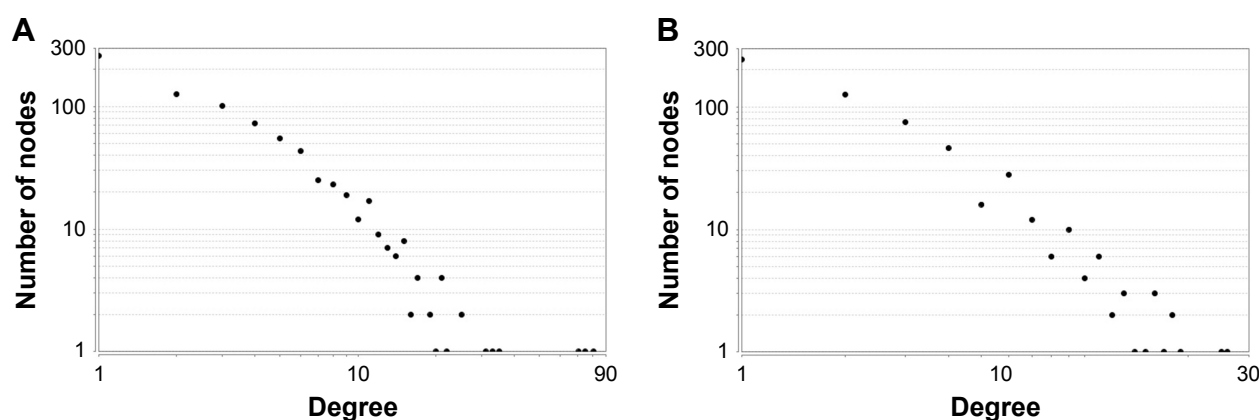
Figure 3 Degree distributions of network nodes.
