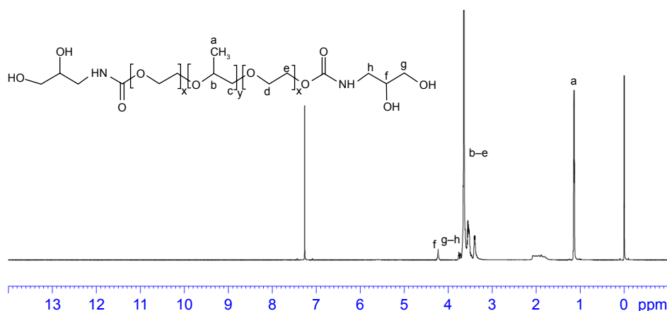
Figure S9 The ^1\text{H} NMR image of F127-APD.
