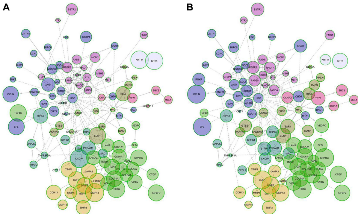
Figure 7 MEN of protein impact score. (A) Control cell lines and (B) cell lines treated with AgNPs.
