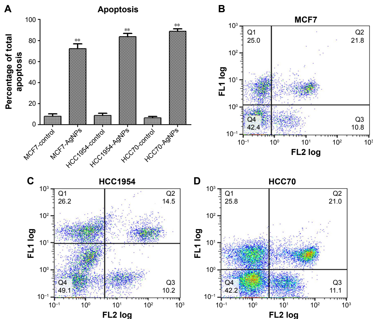
Figure 5 Determination of apoptosis: cells were stained with Annexin V-fluorescein isothiocyanate (FLI) and propidium iodide (FL2), and cell apoptosis was analyzed by flow cytometry. (A) Total apoptosis percentage presented as mean and standard deviation; differences were calculated by the Student's t -test. p < 0.01 (**). (B–D) Dot plots representative of each cell line.
