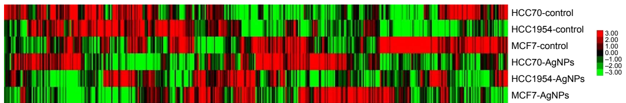
Figure 6 Gene expression heat map of 437 selected genes in each cell line.
