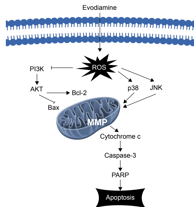
Figure 5 Evo activated apoptosis by suppressing PI3K/AKT and activating MAPKs in glioma cells.
