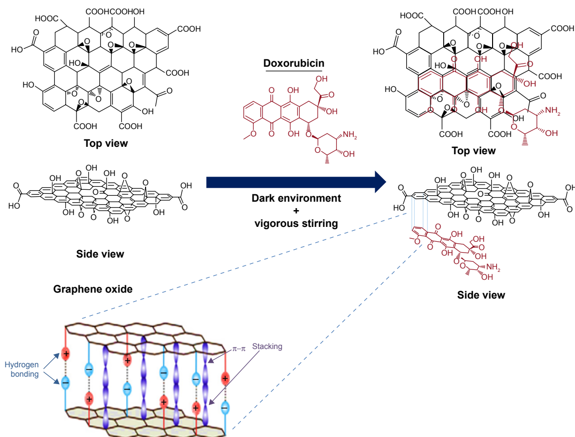
Figure 1 Schematic representation for a graphene oxide–doxorubicin conjugation.
