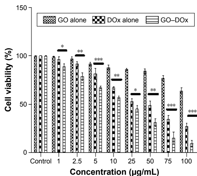
Figure 5 Cytotoxicity of DOx and GO-DOx on the FaDu cell line. * P < 0.05 ; ** P < 0.01 ; *** P < 0.001 , significant when compared to respective controls. Abbreviations: DOx, doxorubicin; GO, graphene oxide.
