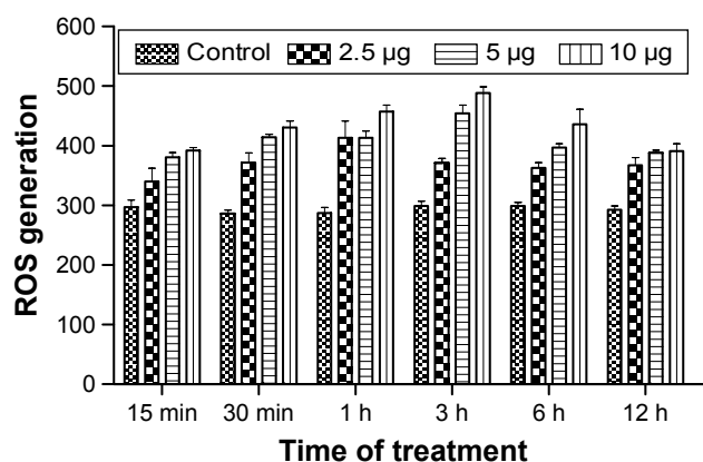
Figure 7 Reactive oxygen species (ROS) generation.
