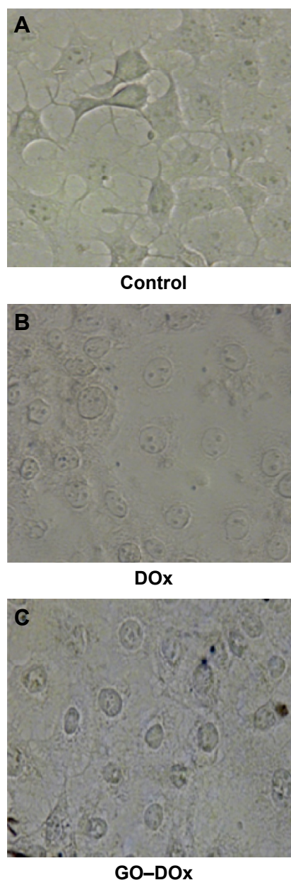
Figure 6 Morphology of FaDu cells (A) untreated and treated with (B) DOx and (C) GO-DOx. Phase contrast microscopy, 40 \times objective. Abbreviations: DOx, doxorubicin; GO, graphene oxide.
