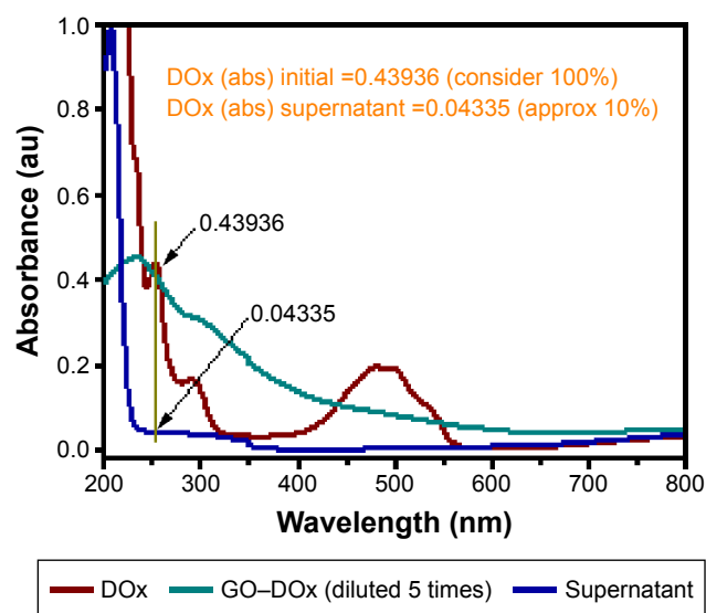
Figure 3 Percent drug (DOx) loaded onto a GO-DOx conjugate.
