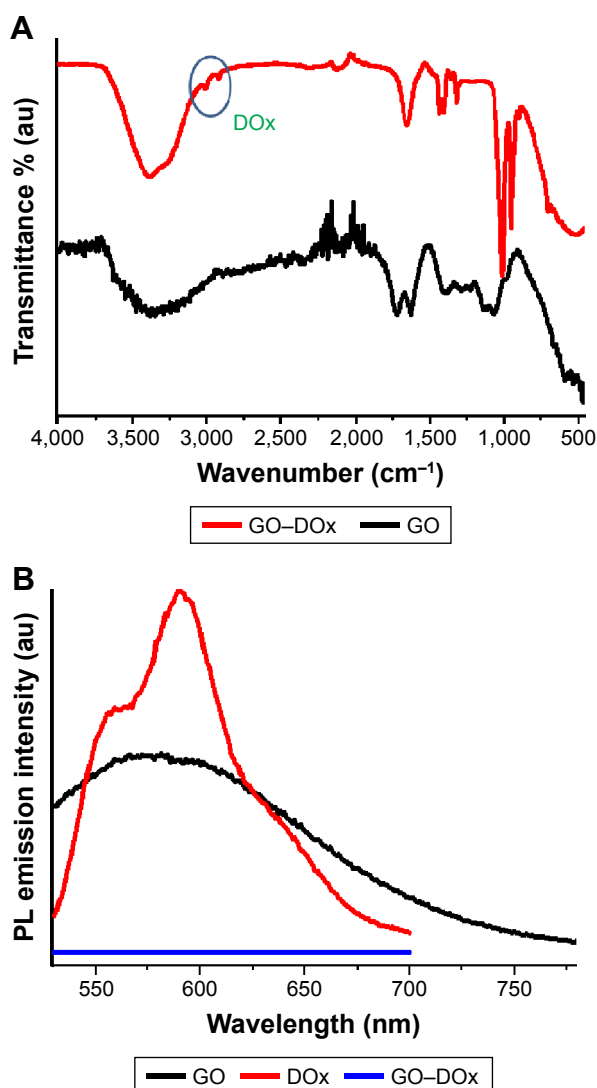
Figure 2 (A) FT-IR spectra showing both GO and GO-DOx conjugate and (B) photoluminescence emission spectra of GO, DOx, and GO-DOx conjugate.
