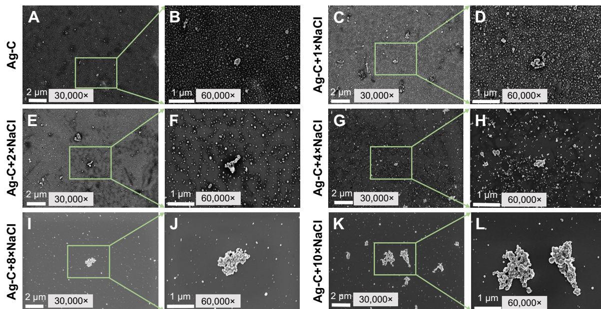
Figure 3 SEM images of the 2 mL Ag-C (A–L) with 200 \mu L different concentrations of NaCl. Abbreviations: SEM, scanning electron microscopy; Ag-C, carbon membrane packaged Ag nanoparticles.
