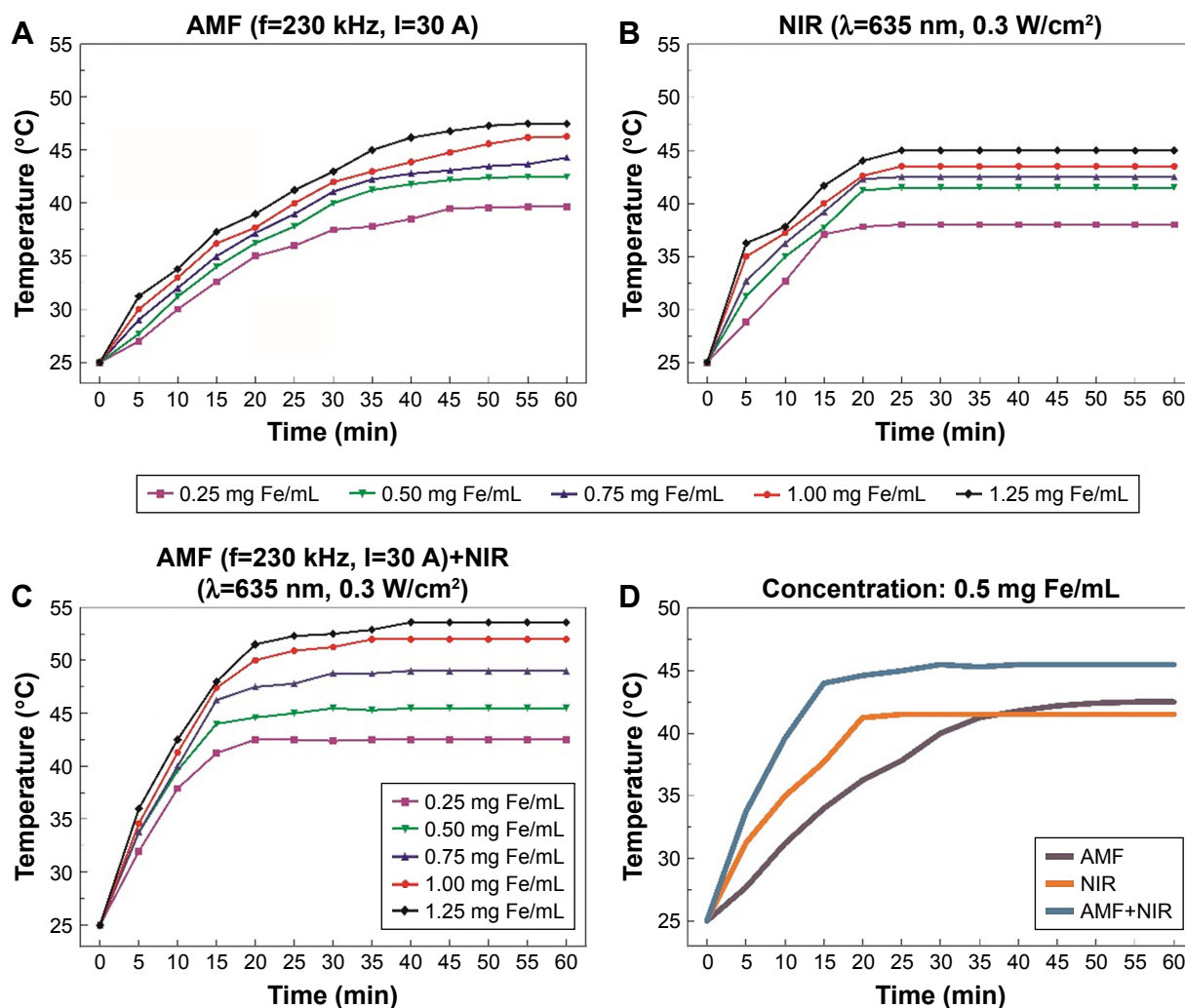
Figure 5 Heat generation by \text{Fe}_3\text{O}_4\text{@Au-C225} MNPs in suspension (0.25–1.25 mg Fe/mL).
