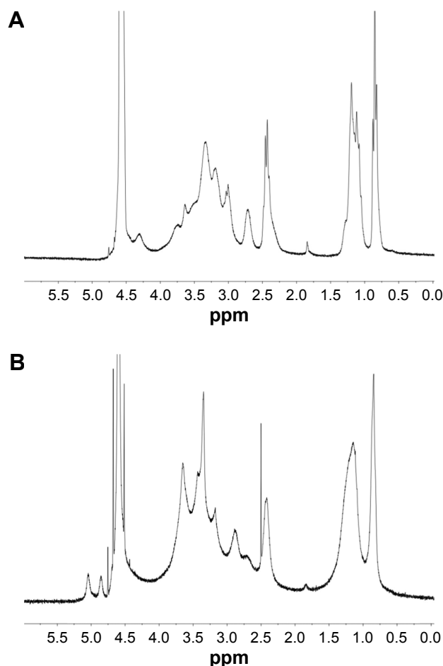
Figure 2 ^1\text{H} -NMR spectra of QA-Ch60 (A) and QA-Ch-MCD (B). Notes: QA-Ch60 (300 MHz, \text{D}_2\text{O} ): \delta = 4.5 (s, anomeric), 4.2–2.2 (m, protons of the pyranosidic ring, methylene protons of pendant quaternized chains -\text{CH}_2\text{CH}_2\text{N}^+(\text{CH}_2\text{CH}_3)_2\text{CH}_2- and -\text{CH}_2\text{N}(\text{CH}_2\text{CH}_3)_2 ), 2.0 (s, methyl protons of N -acetylglucosamine), 1.6–1.1 (m, methyl protons of the ethyl moieties closed to ammonium pendants \text{N}^+\text{CH}_2\text{CH}_3 ), and 1.1–0.8 ppm (m, methyl protons of the terminal part of DEAE chains \text{N}(\text{CH}_2\text{CH}_3)_2 ). QA-Ch-MCD (300 MHz, \text{D}_2\text{O} ) \delta = 5.13 and 4.95 (s, MCD anomeric), 4.2–2.6 (m, protons of the pyranosidic ring, methylene protons of pendant quaternized chains -\text{CH}_2\text{CH}_2\text{N}^+(\text{CH}_2\text{CH}_3)_2\text{CH}_2- and -\text{CH}_2\text{N}(\text{CH}_2\text{CH}_3)_2 , methylene protons closed to the N of the spacer -\text{NHCH}_2(\text{CH}_2)_4\text{CH}_2\text{NH}_2 ); 2.5 (s, methylene protons of not protonated N of the DEAE pendant -\text{CH}_2\text{N}(\text{CH}_2\text{CH}_3)_2 ), 2.0 (s, methyl protons of N -acetylglucosamine), 1.7–1.1 (m, methyl protons of the ethyl moieties close to ammonium pendants \text{N}^+(\text{CH}_2\text{CH}_3)_2 and methylene protons of the central part of spacer chain -\text{NHCH}_2(\text{CH}_2)_4\text{CH}_2\text{NH}_2 ), and 1.0–0.7 ppm (m, methyl protons of the terminal part of DEAE chains -\text{N}(\text{CH}_2\text{CH}_3)_2 ). Compounds in bold correspond to peaks in the spectra. Abbreviations: DEAE, 2-diethylaminoethyl chloride; MCD, methyl- \beta -cyclodextrin; QA-Ch60, quaternary ammonium-chitosan 60; QA-Ch-MCD, methyl- \beta -cyclodextrin-quaternary ammonium chitosan; s, singlet; m, multiplet.
