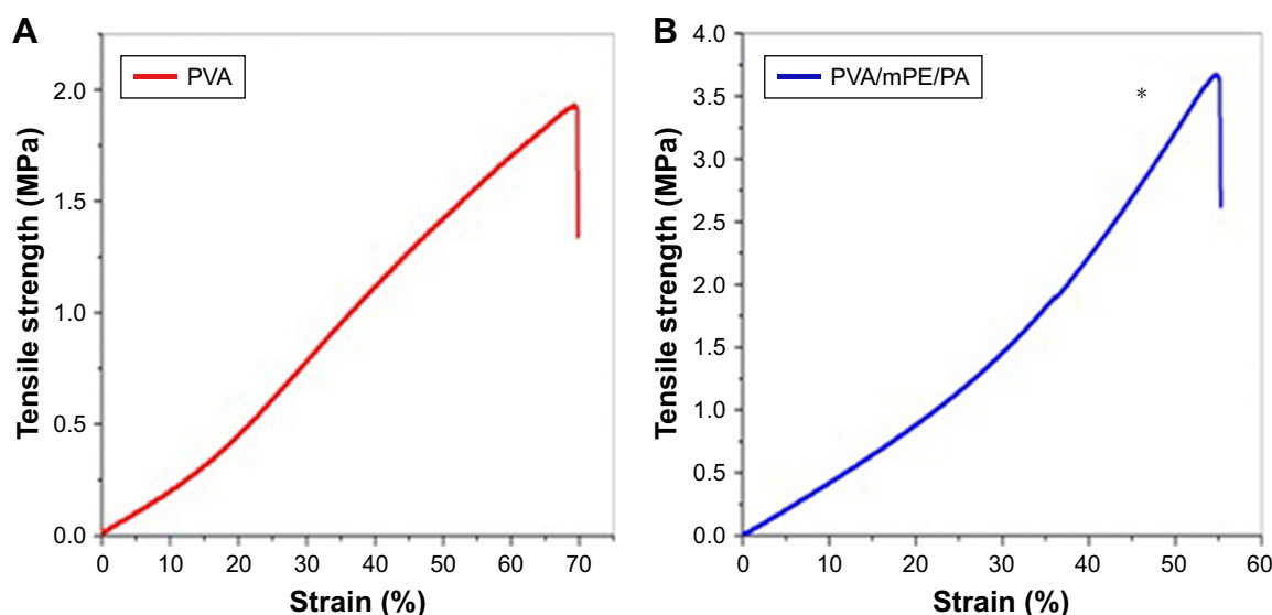
Figure 7 Mechanical testing of (A) PVA membrane and (B) PVA/mPE/PA nanocomposites. Note: *Mean differences were significant compared with pure PVA ( P < 0.05 ). Abbreviations: mPE, metallocene polyethylene; PA, plectranthus amboinicus; PVA, polyvinyl alcohol.
