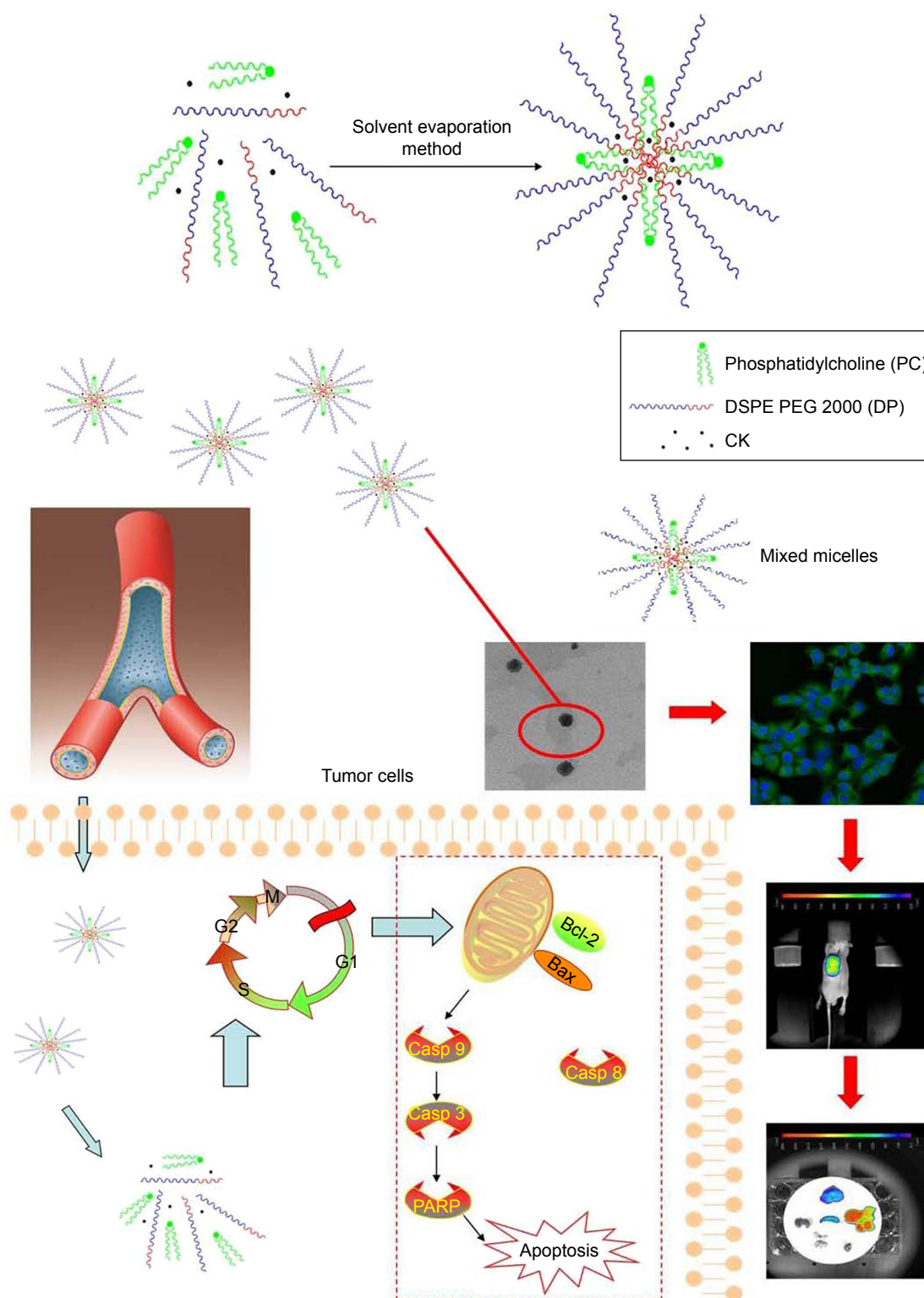
Figure 1 Illustrations of ginsenoside compound-K-based mixed micelles and their mode of action for enhanced antitumor efficacy.
