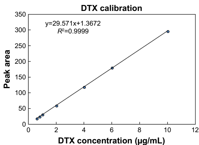
Figure S2 Calibration curve plotted as peak area vs DTX concentration (µg/mL).
