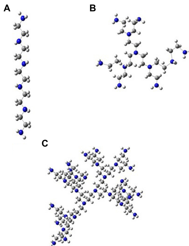
Figure 37 Examples of polyethylenimine molecules: linear (A); branched (B) and dendrimer (C). 216,217*
