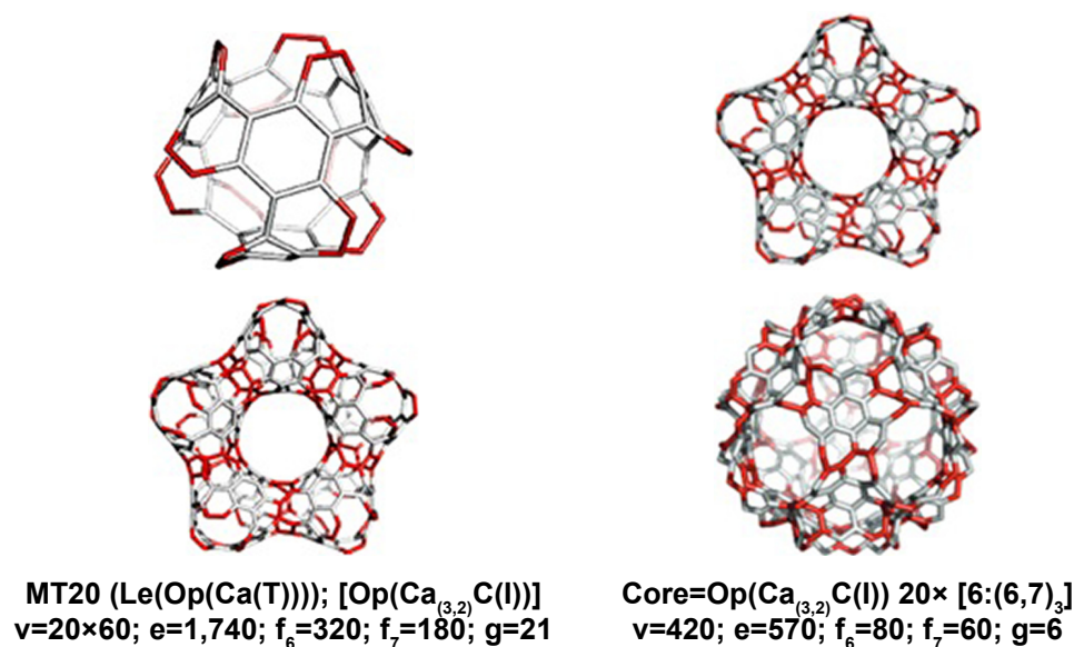
Figure 18 Top row: TriPhen_T_60A (left) and a pentagonal hyper-ring (right). Bottom row: Multi-torus MT(Le(Op(Ca(T)))) [Op(Ca (3,2) C(I)) (left) and its core (right).
