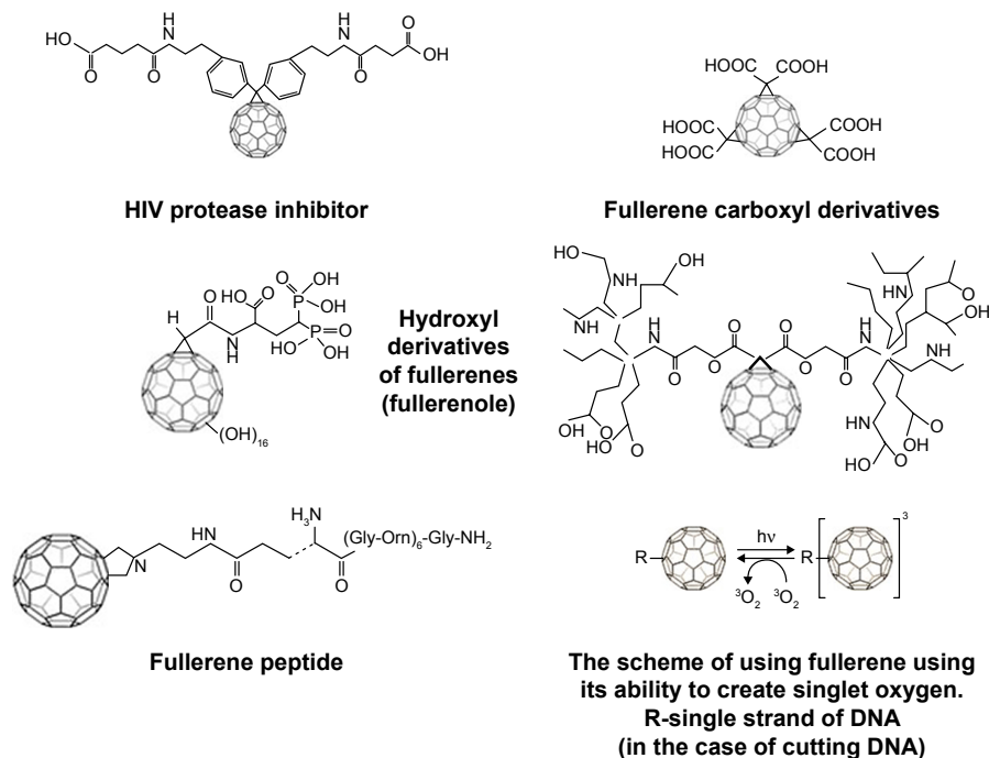
Figure 30 Dendrimers and fullerene derivatives.
