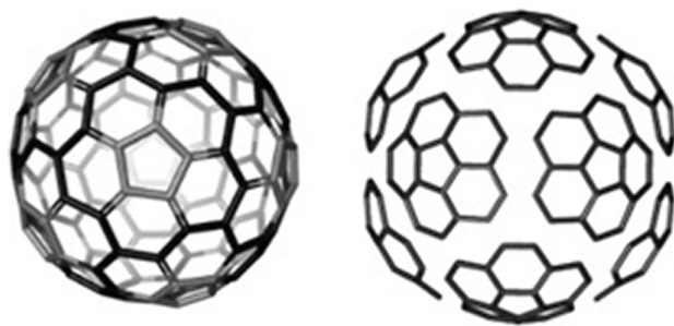
Figure 9 The [5:6] patch in fullerenes: joint patch in C_{140} (left) and disjoint patch in C_{240} (right).
