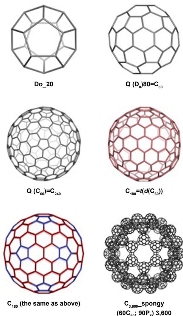
Figure 2 Fullerenes and a hyper-fullerene (bottom right corner).
