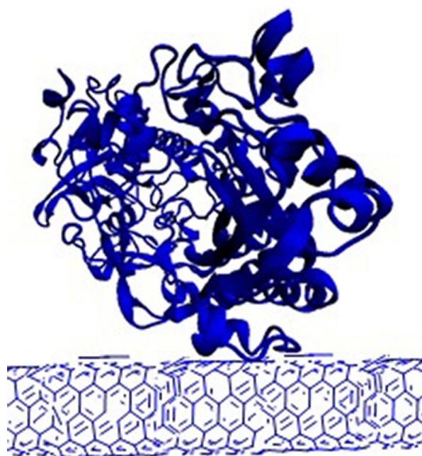
Figure 36 Equilibrated structure of the SWNT-PSE-GOX complex. 199
