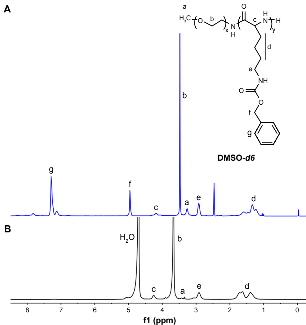
Figure S2 ^1\text{H} NMR spectra of PEG- b -PLLZ in DMSO- d 6 ( A ) and PEG- b -PLL ( B ) in \text{D}_2\text{O} .
