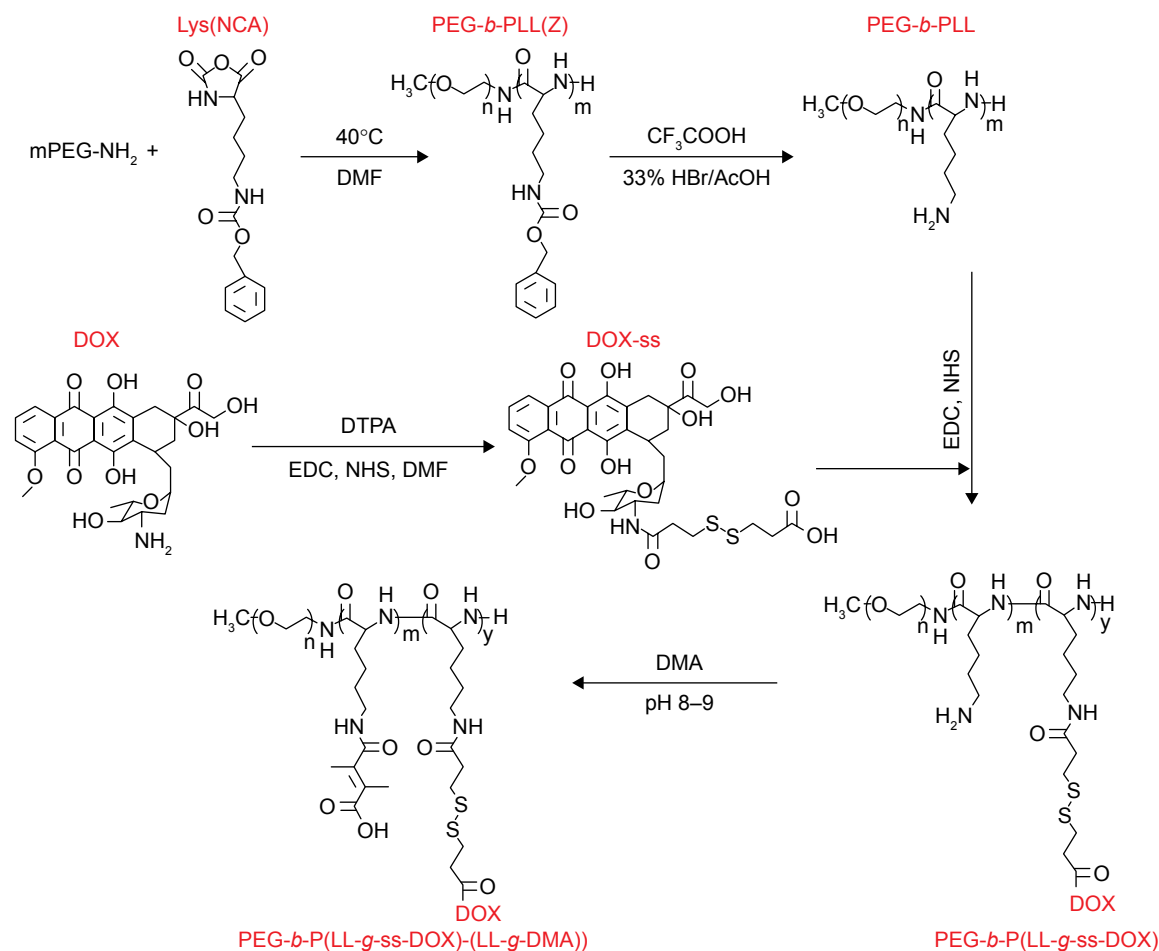
Scheme S1 The synthesis route of PEG- b -P((LL- g -ss-DOX)-(LL- g -DMA)).
