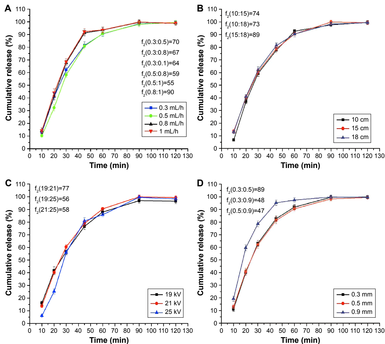
Figure 2 The influence of electrospray process parameters on drug dissolution in a 0.5% Tween 80 pH 6.8 medium dissolution. (A) The effect of solution feed rate; (B) the effect of distance; (C) the effect of voltage; (D) the effect of needle inner diameter.
