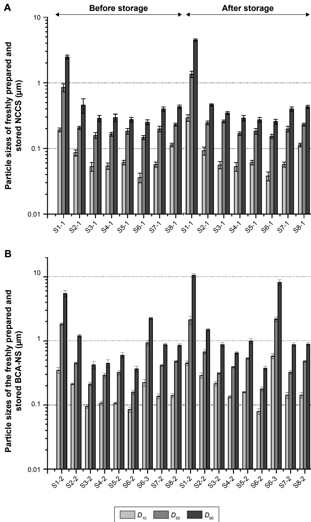
Figure 3 Particle sizes of NCCS ( A ) and BCA-NS/NCCS ( B ) before and after storage.
