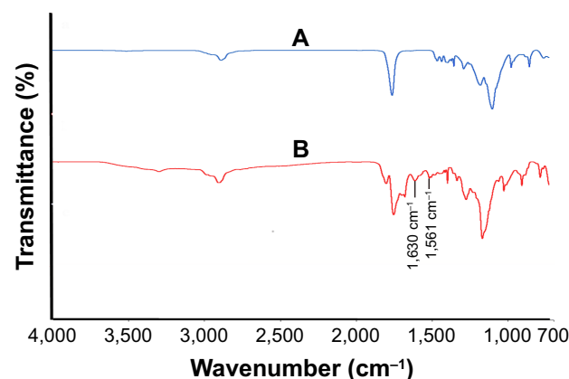
Figure 4 Fourier-transform infrared spectra of (A) unconjugated PLGA NP and (B) K4 peptide-conjugated PLGA NP.
