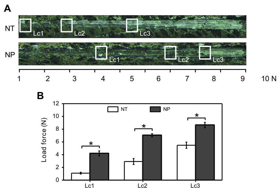
Figure 2 (A) Representative scratch track image of NT and NP; (B) statistics of critical loads of cohesion (Lc1), adhesion (Lc2) and breakthrough (Lc3). Error bars represent mean \pm SD for n=4, * p <0.05.
