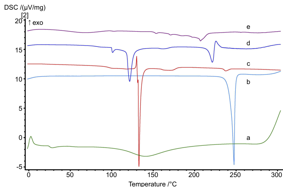
Figure 3 DSC thermograms of (a) CS, (b) PA, (c) SD, (d) F12 ingredients physical mixture, and (e) F12 NPs formulation.
