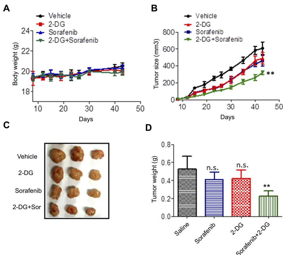
Figure 6 2-DG combined with sorafenib exhibits antitumor effects in persisting cell xenograft tumors in vivo. (A) The body weight of Hep3B-P human liver cancer xenografts in nude mice after treatment with the indicated drugs for 43 days. (B) The tumor volume, (C) tumor image and (D) tumor weight of Hep3B-P human liver cancer xenografts in nude mice after treatment with the indicated drugs for 43 days. Bars, means \pm SD. ** p < 0.01 , n = 5 .
