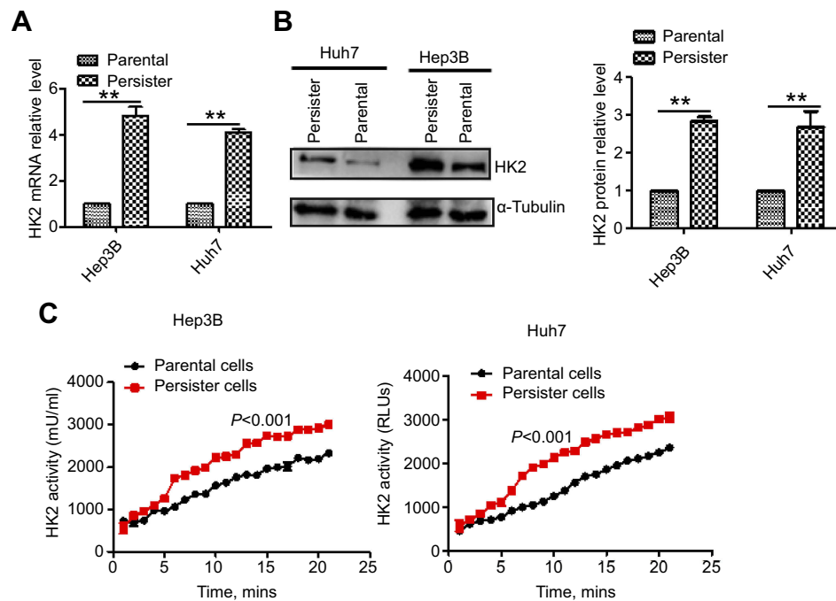
Figure 3 HK2 high expression in persister cells. (A) Comparison of the mRNA expression of glycolytic enzyme HK2 in parental and persister cells by real-time PCR analysis. Bars, means \pm SEM. **p < 0.01 , n = 3 . (B) Immunoblotting analysis of the major glycolytic enzymes in parental and persister cells. (C) A HK2 enzyme activity assay in HK2 in parental and persister cells was performed as described in the Materials and methods section. The results were statistically significant ( p < 0.001 ).
