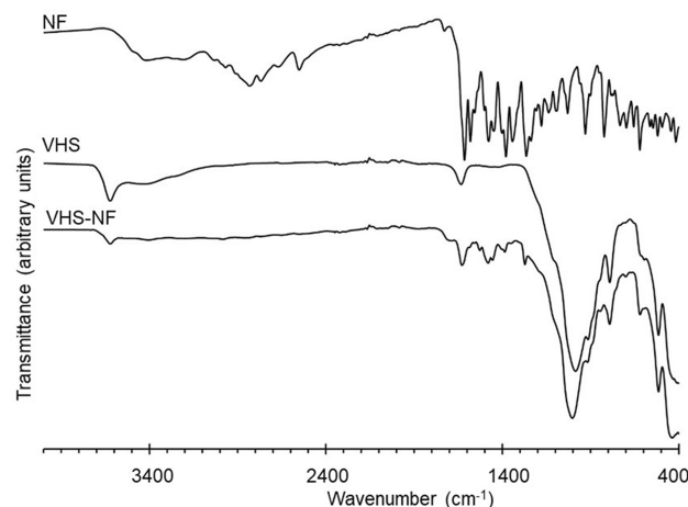
Figure 3 FT-IR spectra of NF, VHS and VHS-NF.
