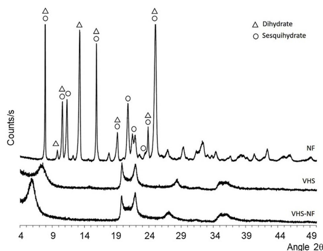
Figure 2 XRPD diffraction patterns of NF, VHS and VHS-NF.
