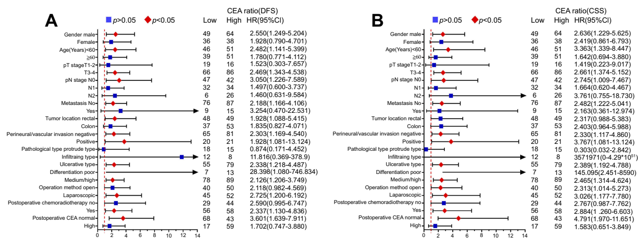
Figure 3 Subgroup multivariate analysis of CEA ratio on each baseline feature in DFS (A), CSS (B).
