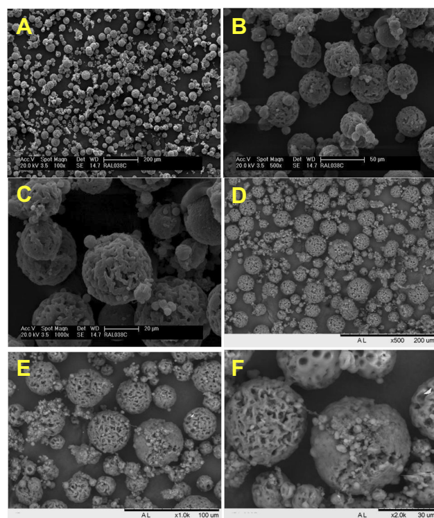
Figure 2 SEM images of PHB-HV 8%-MS in Philips XL30 Microscope (A–C) and Tabletop Microscope TM3000 (D–F). Magnifications: (A) 100×, (B) 500×, (C) 1000×, (D) 500×, (E) 1000×, and (F) 2000×.
