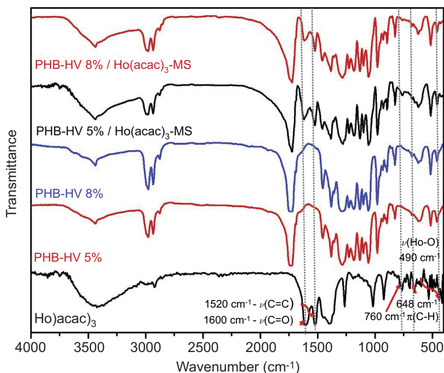
Figure 8 Infrared spectra of raw materials, polyesters, and micromaterials.
